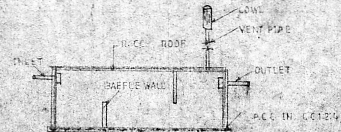
SECTION OF SEPTIC TANK
